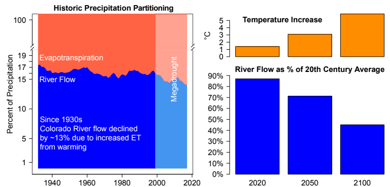
Fig. 1. Climate change is causing the Southwest to aridify. (Left) Since the 1930s, increasing temperatures have caused the percentage of precipitation going to evapotranspiration (ET) to increase at the expense of precipitation going to Colorado River flow, resulting in an unprecedented and still ongoing megadrought (shading) starting in 1999 (8). (Right) Higher temperatures have already reduced Colorado River flow by 13%, and projected additional warming, assuming continued high emissions of greenhouse gases, will increase ET while reducing river flow even more through the 21st century. Data on Left are 20-y running means from ref. 5, and data on Right are calculated from Representative Concentration Pathways (RCP) 8.5 multimodel Coupled Model Intercomparison Project–Phase 5 (CMIP5) ensemble temperature increases projected for the Upper Colorado River Basin combined with temperature sensitivity of -9.3\%/^{\circ}\text{C} estimated by ref. 5, assuming no change in precipitation.
